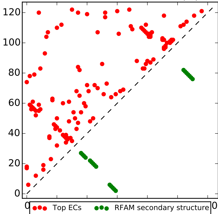
Top L contacts for RF00420 with |i-j| > 4
