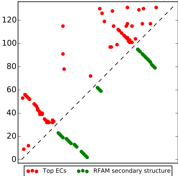
Top L/2 contacts for RF00425 with |i-j| > 4
