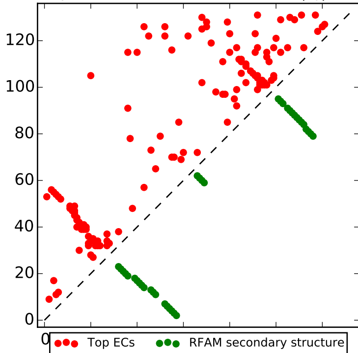
Top L contacts for RF00425 with |i-j| > 4
