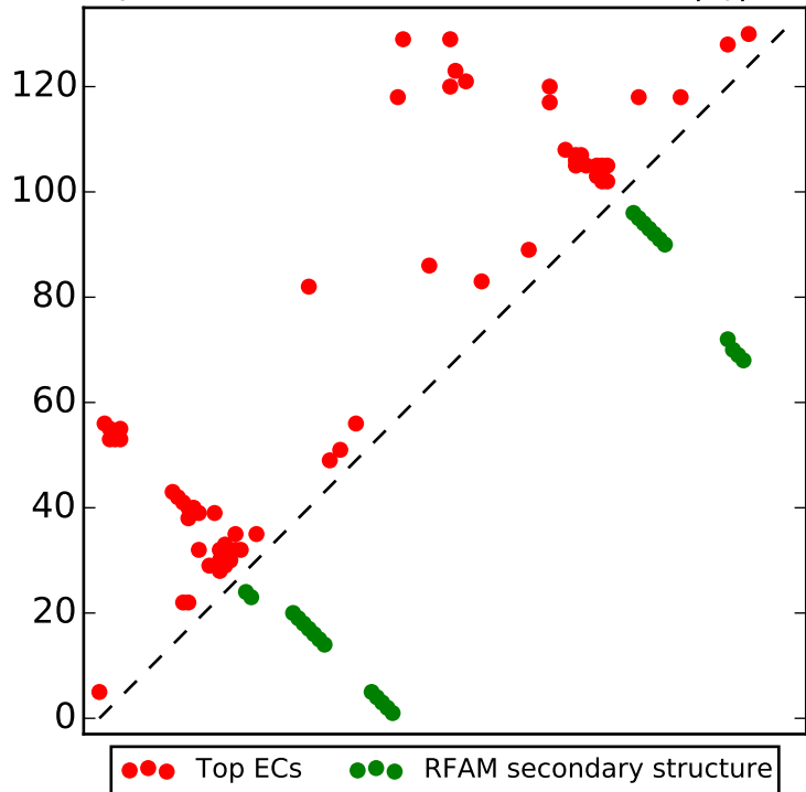
Top L/2 contacts for RF00428 with |i-j| > 4
