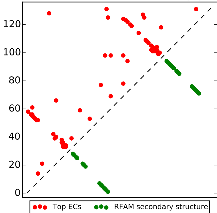
Top L/2 contacts for RF00432 with |i-j| > 4
