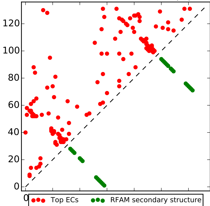
Top L contacts for RF00432 with |i-j| > 4
