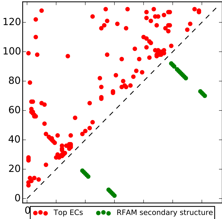
Top L contacts for RF00438 with |i-j| > 4
