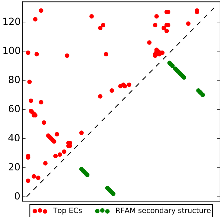
Top L/2 contacts for RF00438 with |i-j| > 4
