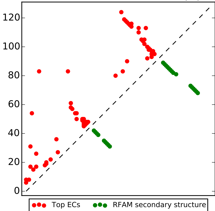
Top L/2 contacts for RF00443 with |i-j| > 4
