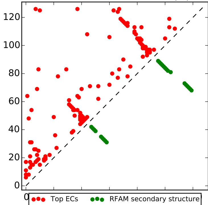
Top L contacts for RF00443 with |i-j| > 4
