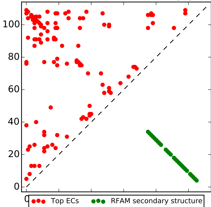
Top L contacts for RF00445 with |i-j| > 4
