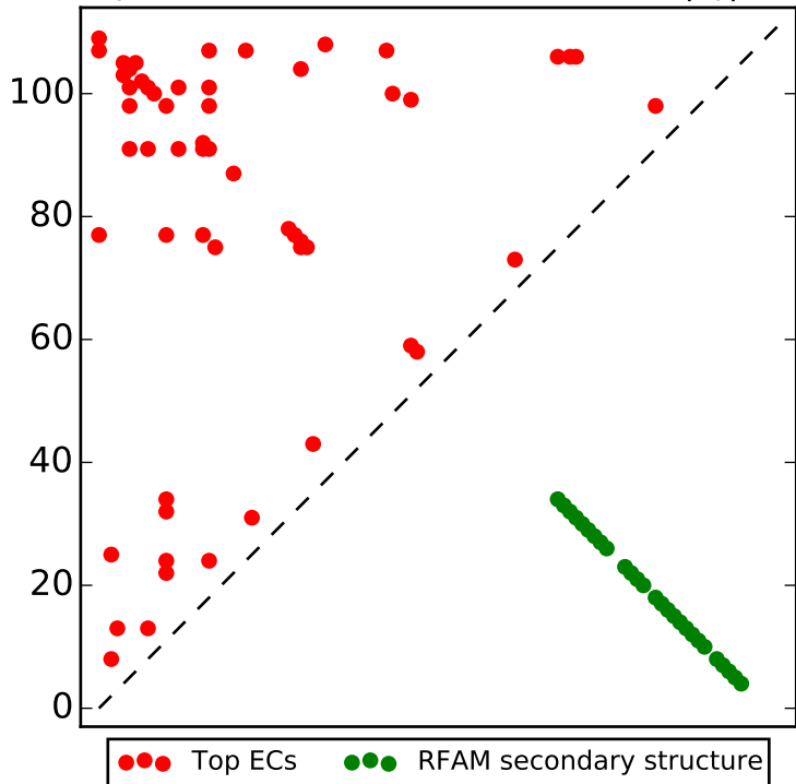
Top L/2 contacts for RF00445 with |i-j| > 4
