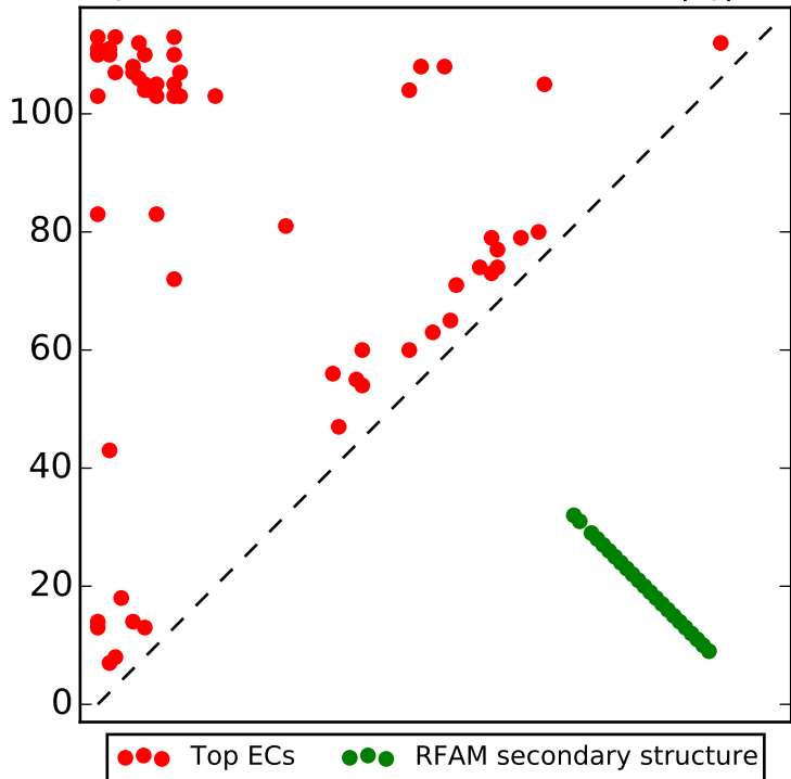
Top L/2 contacts for RF00452 with |i-j| > 4
