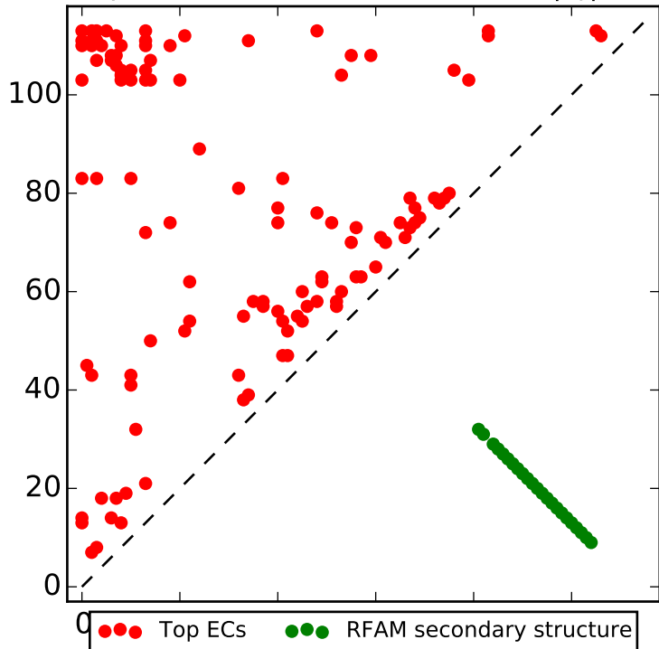
Top L contacts for RF00452 with |i-j| > 4
