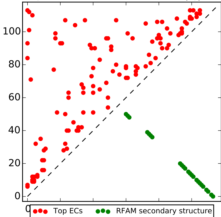
Top L contacts for RF00485 with |i-j| > 4
