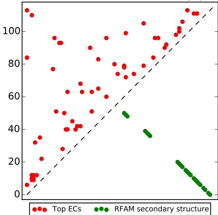
Top L/2 contacts for RF00485 with |i-j| > 4
