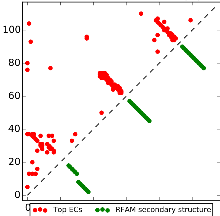
Top L contacts for RF00515 with |i-j| > 4
