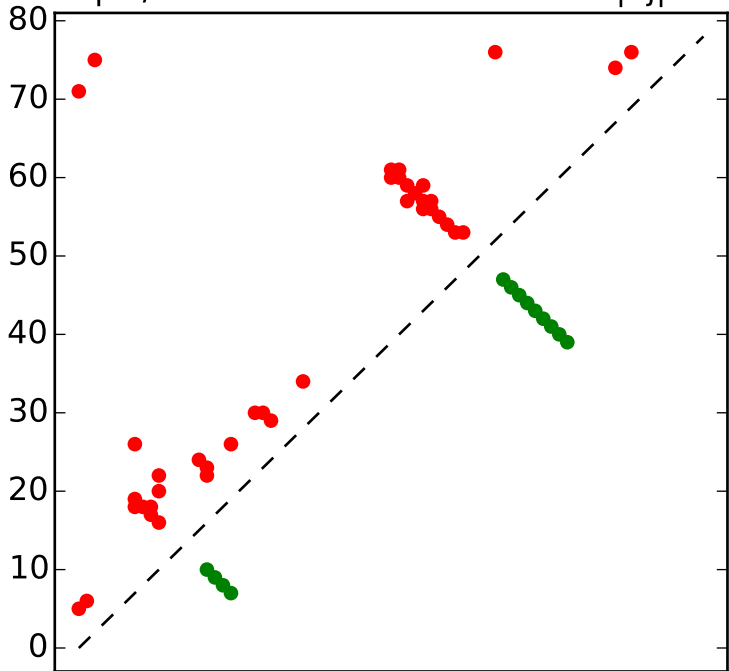
Top L/2 contacts for RF00519 with |i-j| > 4
