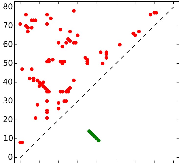
Top L contacts for RF00521 with |i-j| > 4
