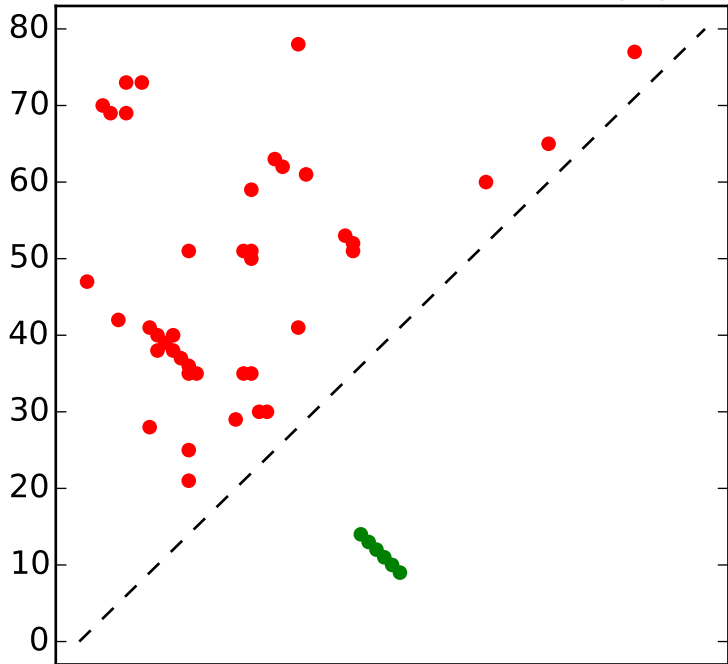
Top L/2 contacts for RF00521 with |i-j| > 4
