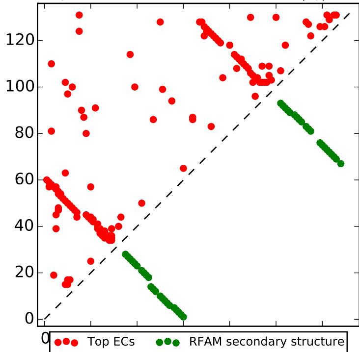
Top L contacts for RF00560 with |i-j| > 4
