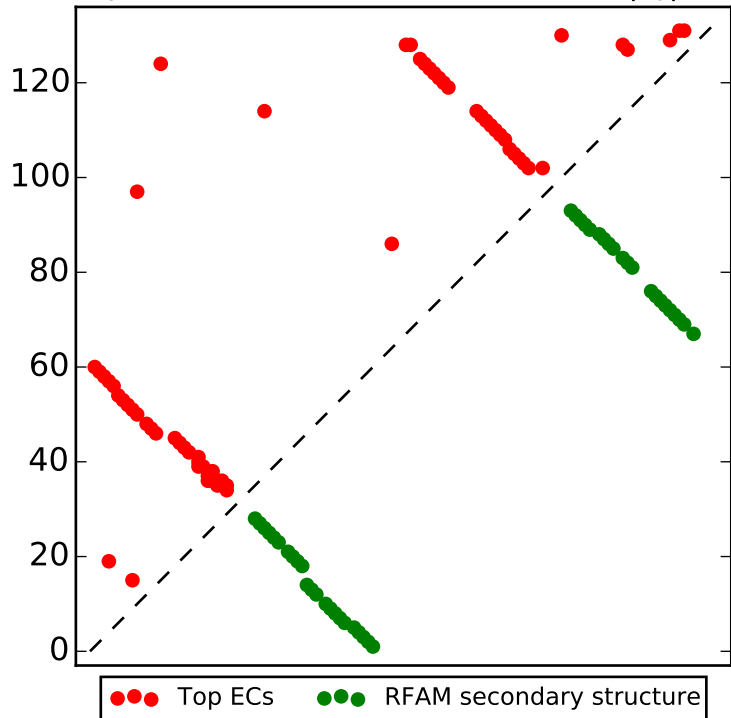
Top L/2 contacts for RF00560 with |i-j| > 4
