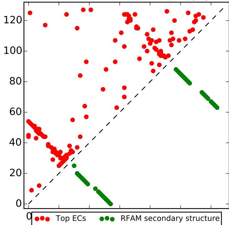
Top L contacts for RF00561 with |i-j| > 4
