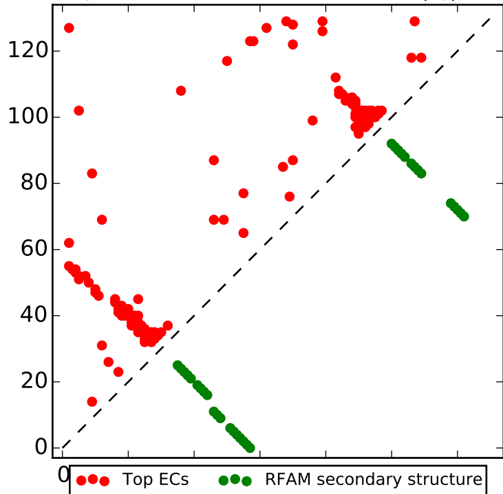
Top L contacts for RF00601 with |i-j| > 4
