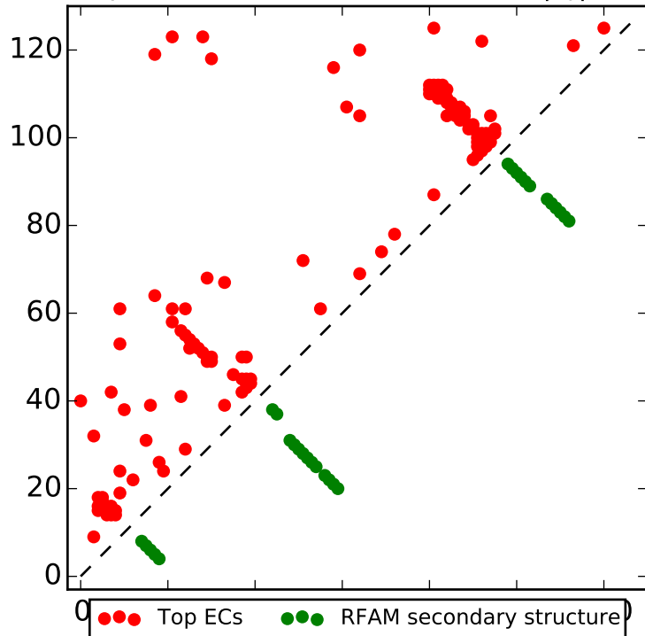
Top L contacts for RF00618 with |i-j| > 4
