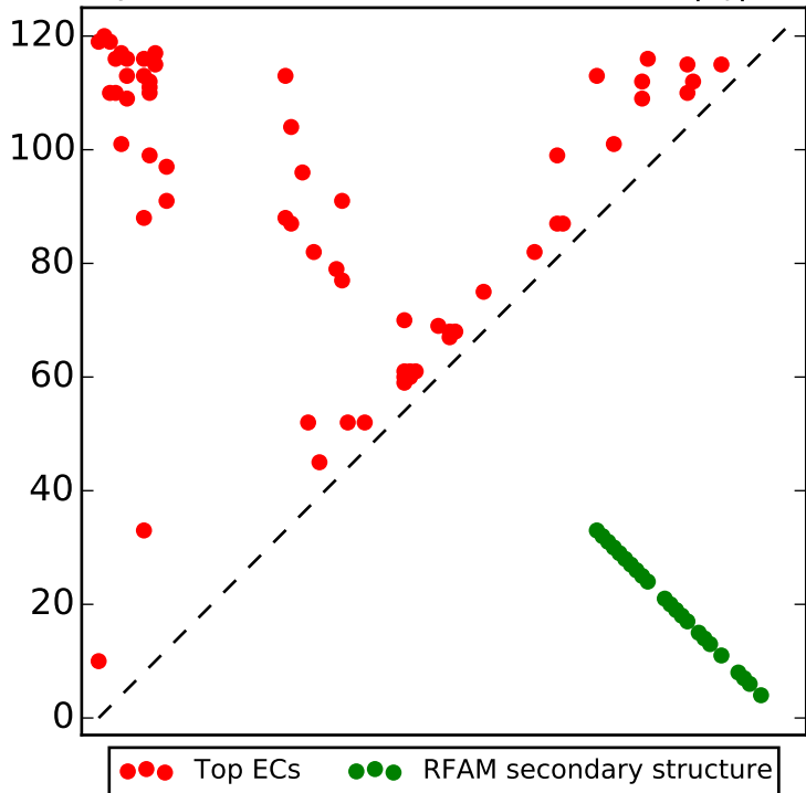
Top L/2 contacts for RF00640 with |i-j| > 4
