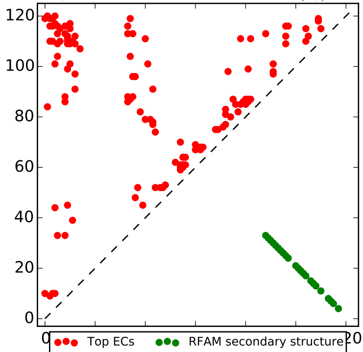
Top L contacts for RF00640 with |i-j| > 4
