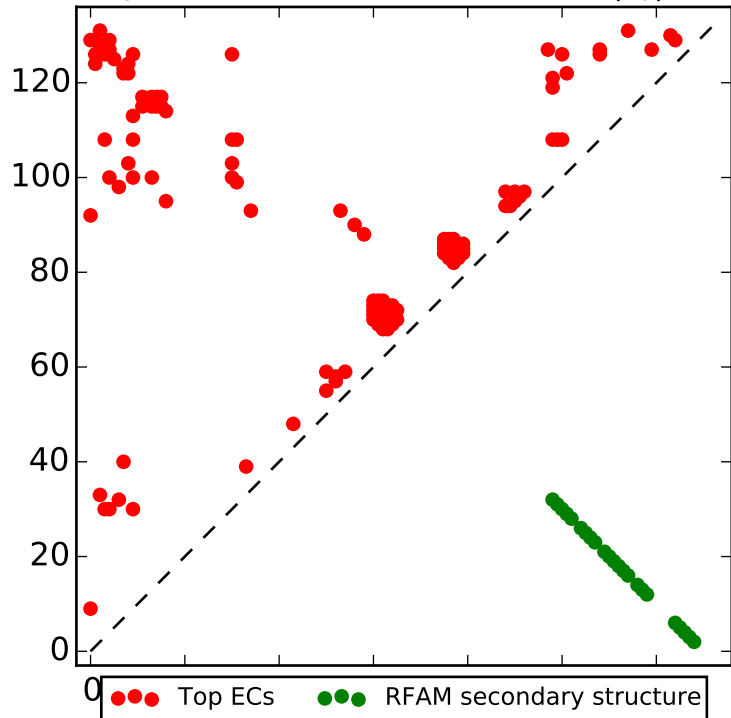
Top L contacts for RF00648 with |i-j| > 4
