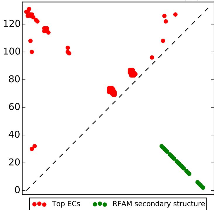
Top L/2 contacts for RF00648 with |i-j| > 4
