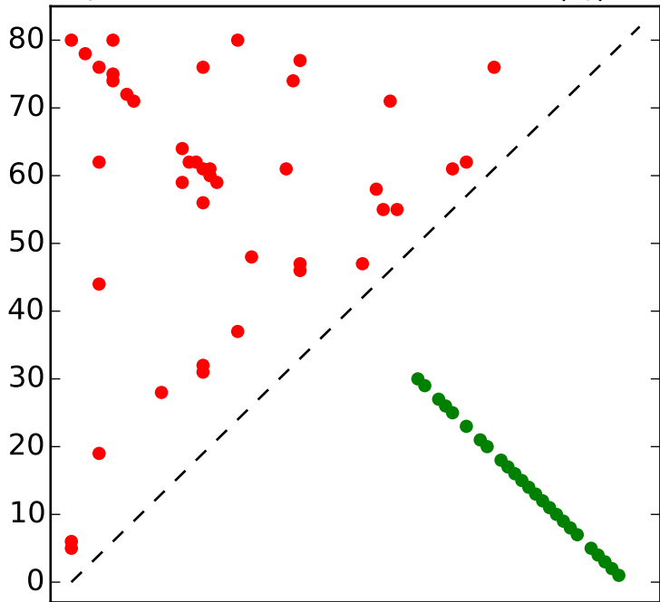
Top L/2 contacts for RF00665 with |i-j| > 4
