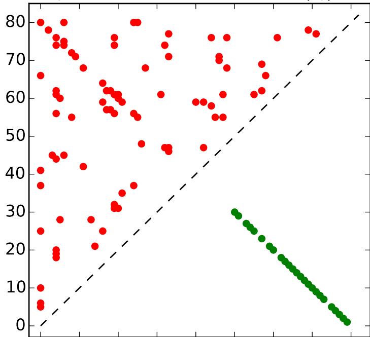
Top L contacts for RF00665 with |i-j| > 4
