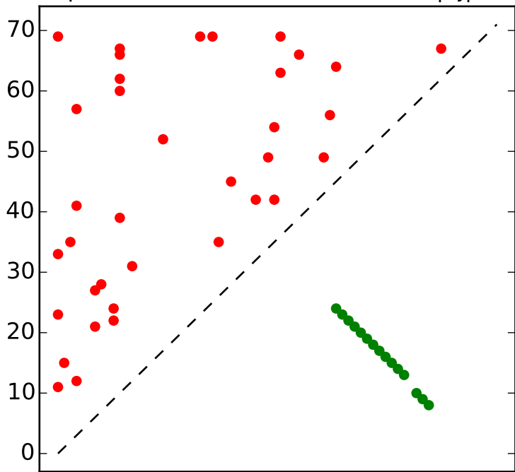
Top L/2 contacts for RF00693 with |i-j| > 4
