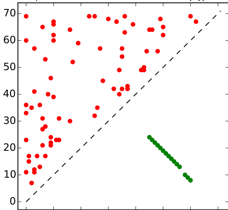
Top L contacts for RF00693 with |i-j| > 4
