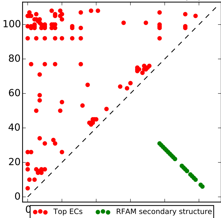
Top L contacts for RF00695 with |i-j| > 4
