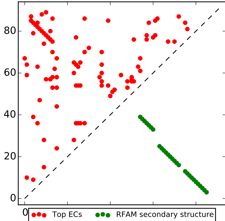
Top L contacts for RF00711 with |i-j| > 4
