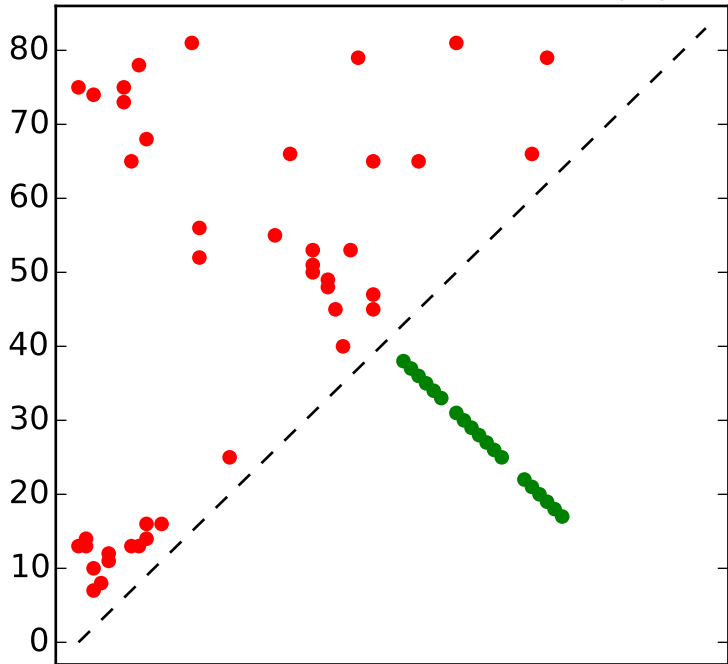
Top L/2 contacts for RF00736 with |i-j| > 4
