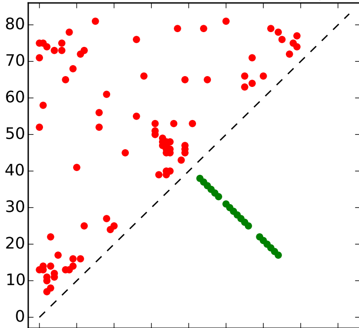
Top L contacts for RF00736 with |i-j| > 4
