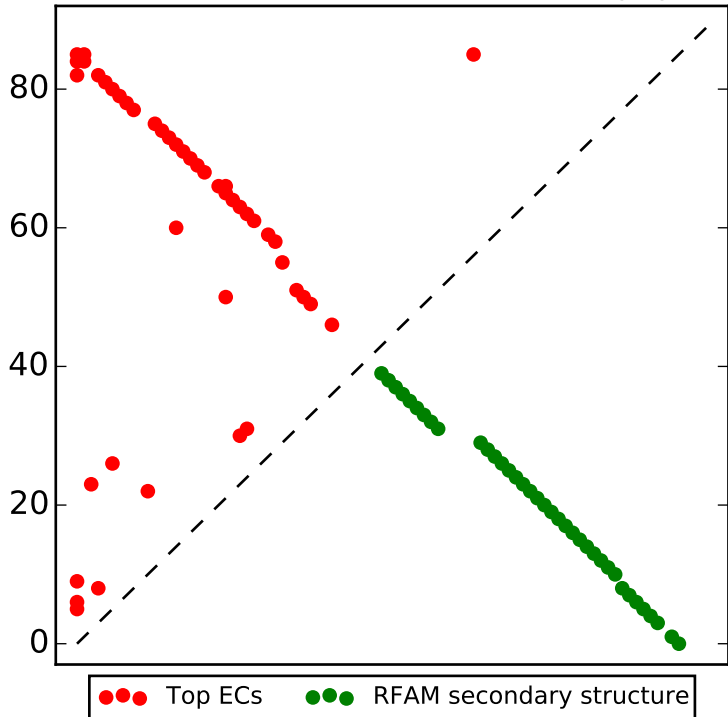
Top L/2 contacts for RF00779 with |i-j| > 4
