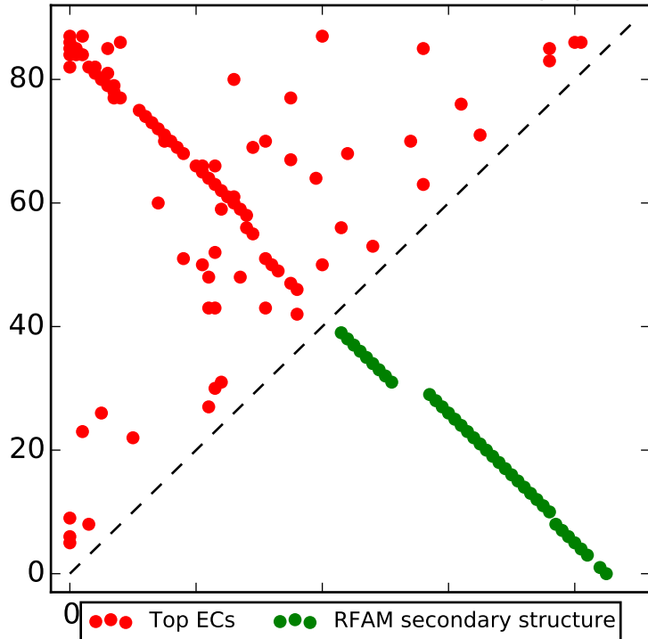
Top L contacts for RF00779 with |i-j| > 4
