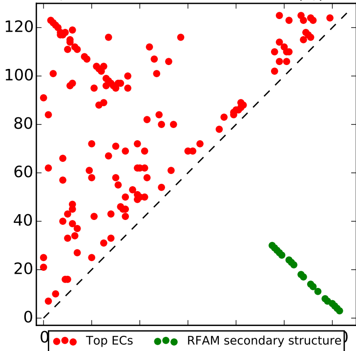
Top L contacts for RF00782 with |i-j| > 4
