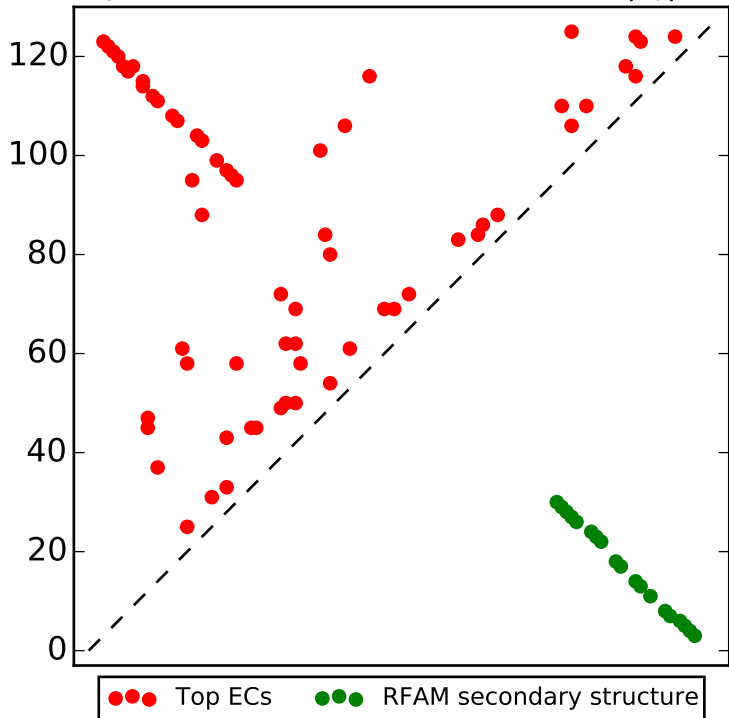
Top L/2 contacts for RF00782 with |i-j| > 4
