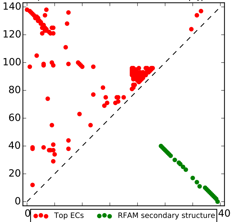
Top L contacts for RF00865 with |i-j| > 4
