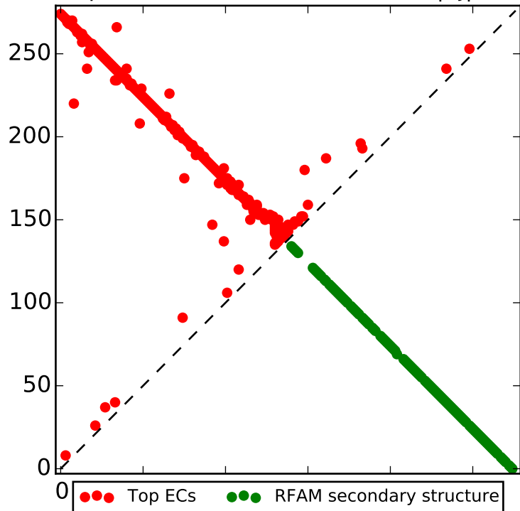
Top L contacts for RF00885 with |i-j| > 4
