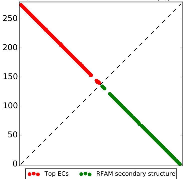
Top L/2 contacts for RF00885 with |i-j| > 4
