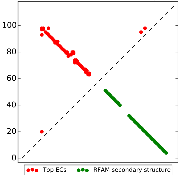
Top L/2 contacts for RF00906 with |i-j| > 4
