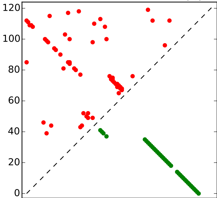
Top L/2 contacts for RF01016 with |i-j| > 4
