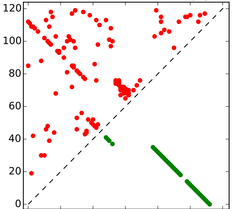
Top L contacts for RF01016 with |i-j| > 4
