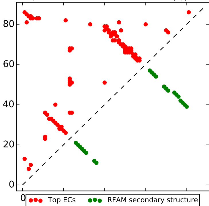
Top L contacts for RF01051 with |i-j| > 4
