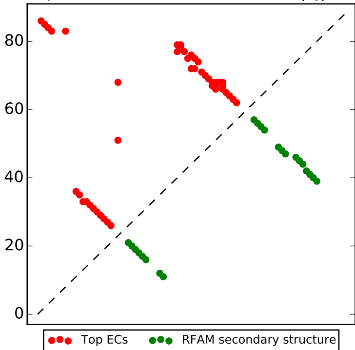
Top L/2 contacts for RF01051 with |i-j| > 4
