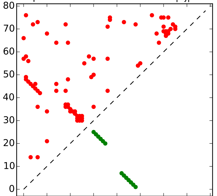
Top L contacts for RF01057 with |i-j| > 4
