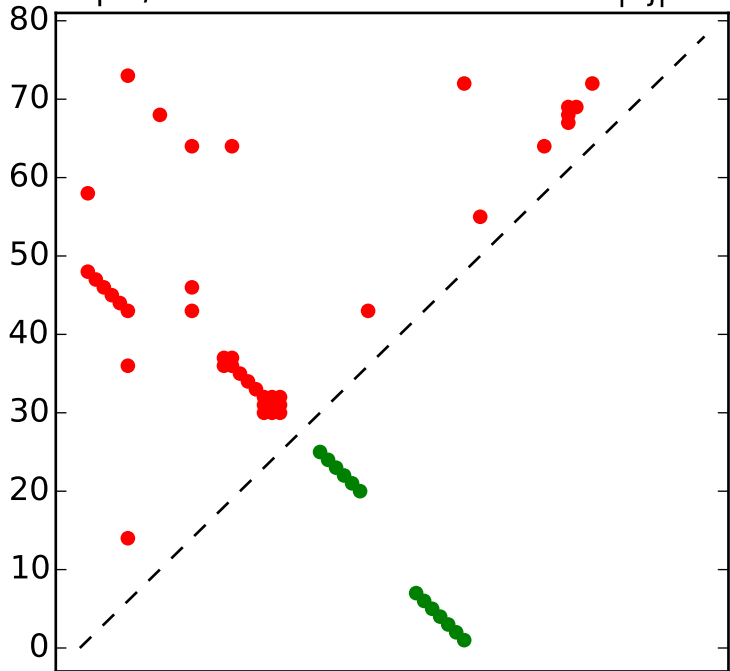
Top L/2 contacts for RF01057 with |i-j| > 4
