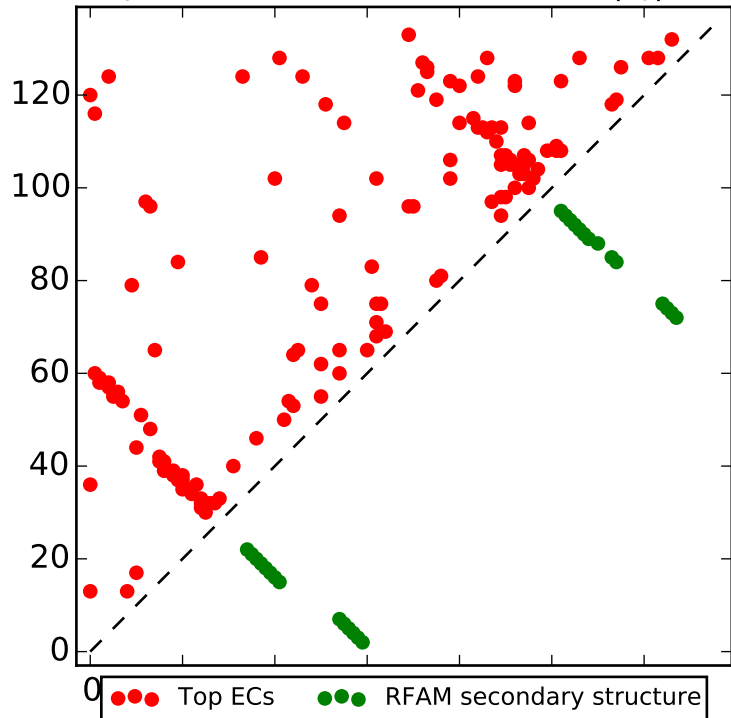
Top L contacts for RF01233 with |i-j| > 4
