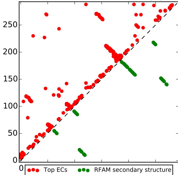
Top L contacts for RF01417 with |i-j| > 4
