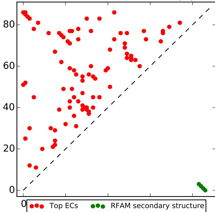
Top L contacts for RF01421 with |i-j| > 4
