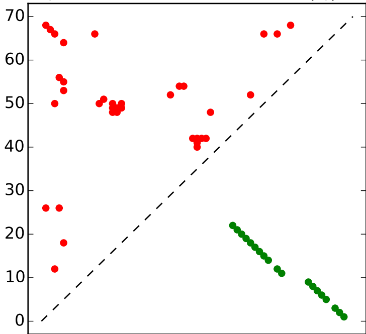
Top L/2 contacts for RF01656 with |i-j| > 4
