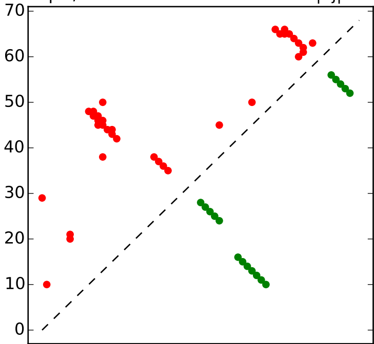
Top L/2 contacts for RF01690 with |i-j| > 4
