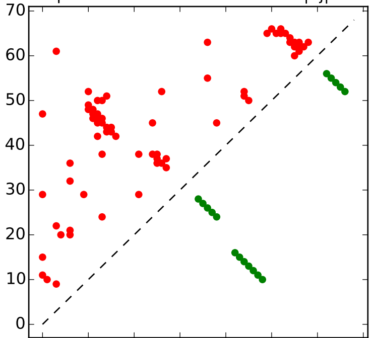
Top L contacts for RF01690 with |i-j| > 4
