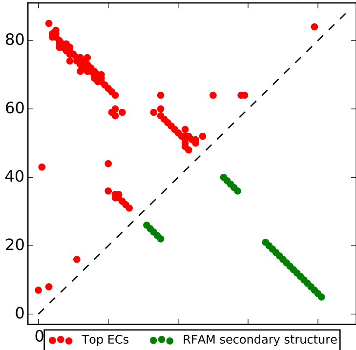
Top L contacts for RF01695 with |i-j| > 4
