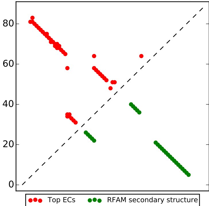
Top L/2 contacts for RF01695 with |i-j| > 4
