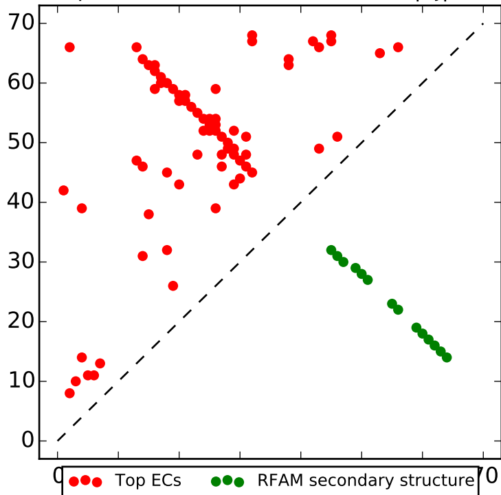
Top L contacts for RF01701 with |i-j| > 4
