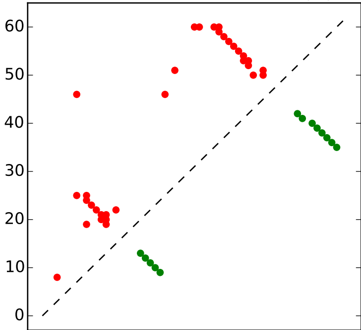
Top L/2 contacts for RF01704 with |i-j| > 4
