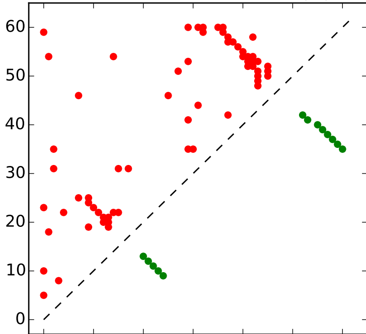
Top L contacts for RF01704 with |i-j| > 4
