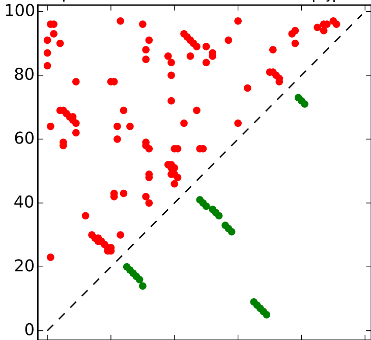
Top L contacts for RF01725 with |i-j| > 4
