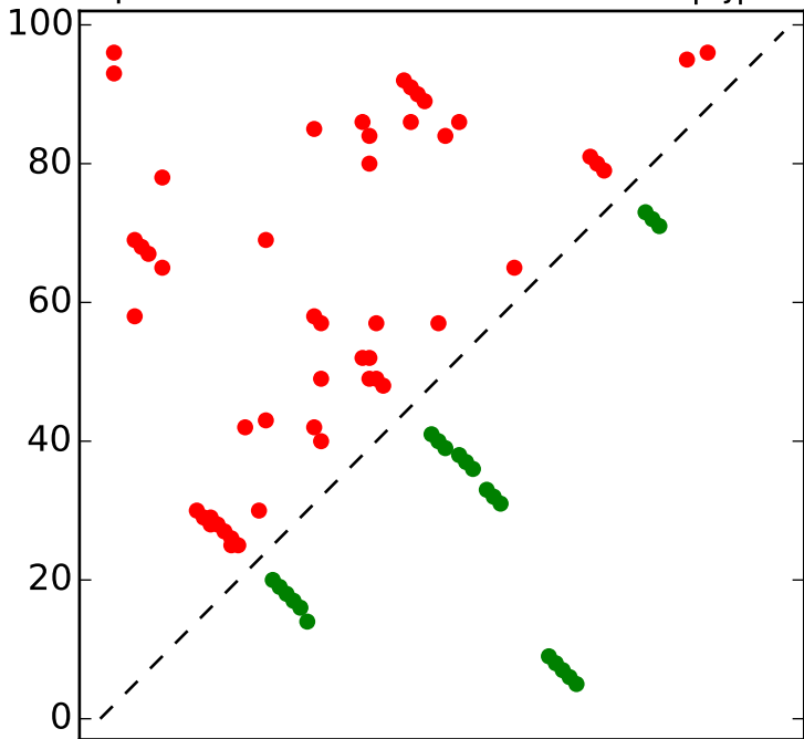
Top L/2 contacts for RF01725 with |i-j| > 4
