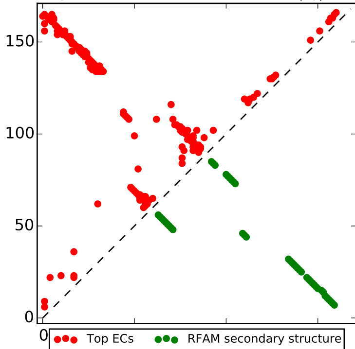
Top L contacts for RF01731 with |i-j| > 4
