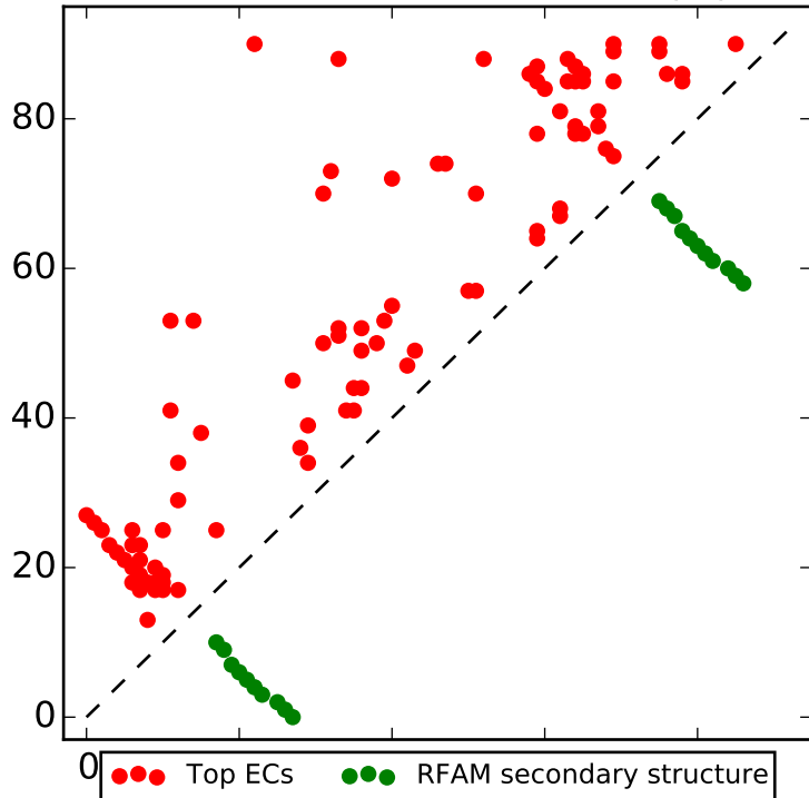
Top L contacts for RF01749 with |i-j| > 4
