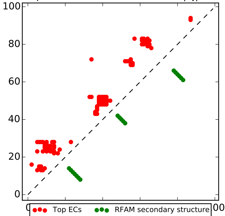
Top L contacts for RF01761 with |i-j| > 4
