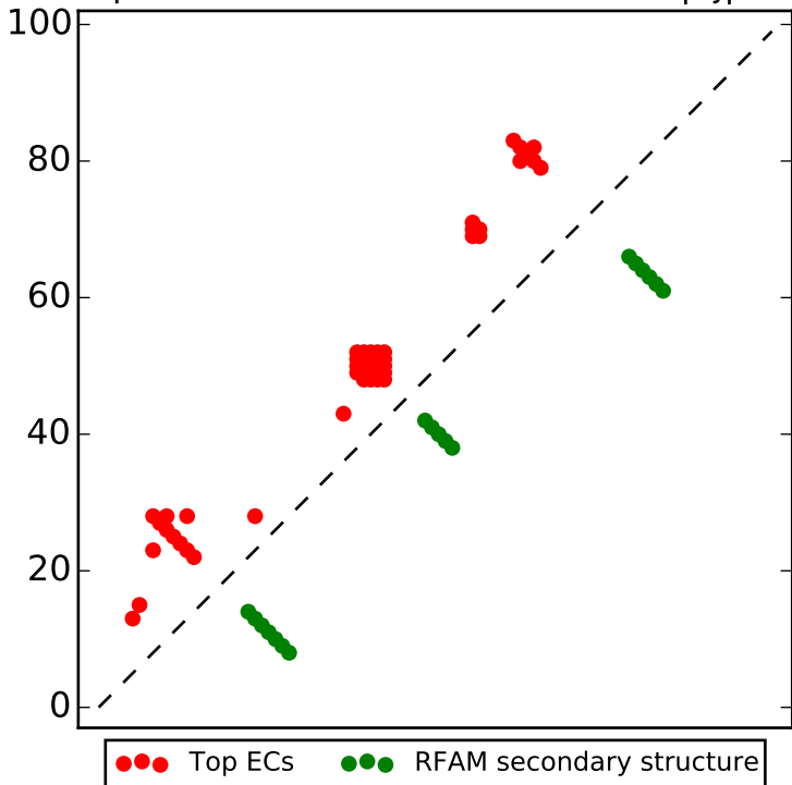
Top L/2 contacts for RF01761 with |i-j| > 4
