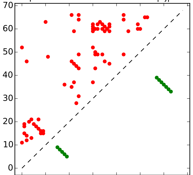
Top L contacts for RF01763 with |i-j| > 4
