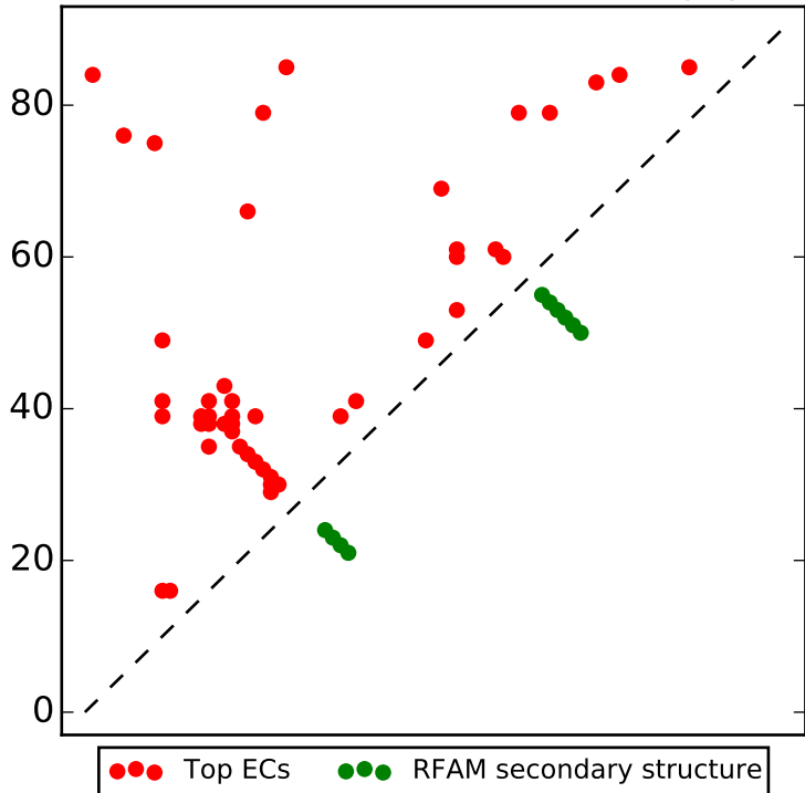
Top L/2 contacts for RF01776 with |i-j| > 4
