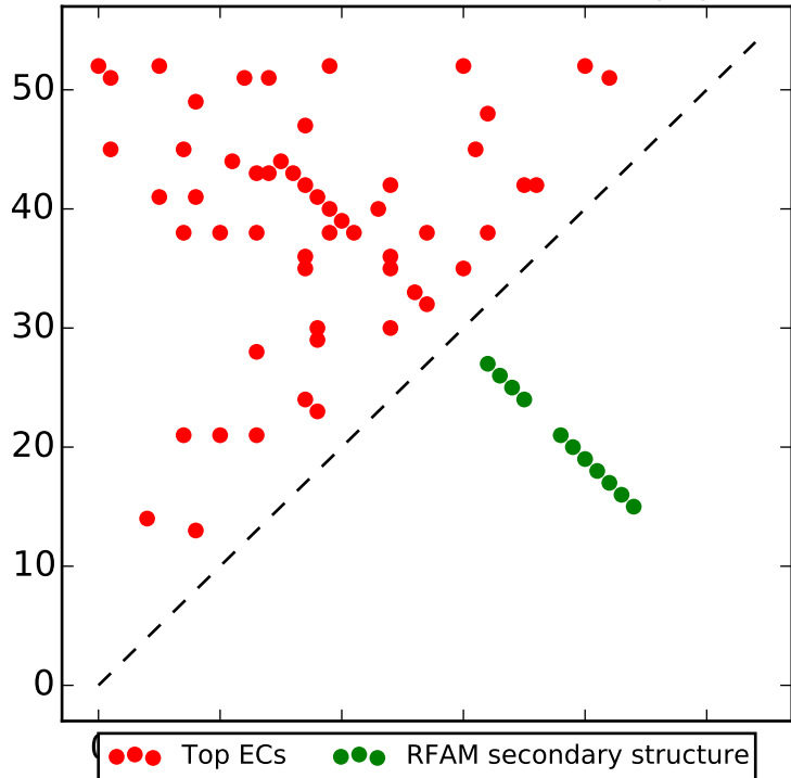
Top L contacts for RF01793 with |i-j| > 4
