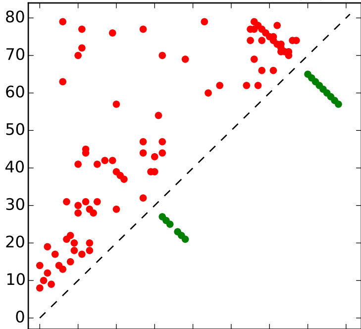
Top L contacts for RF01844 with |i-j| > 4
