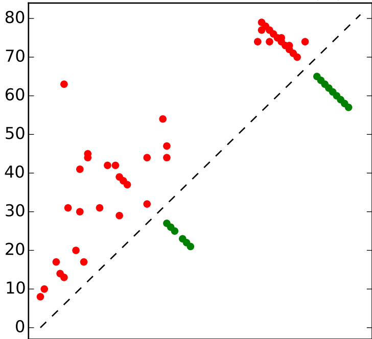
Top L/2 contacts for RF01844 with |i-j| > 4
