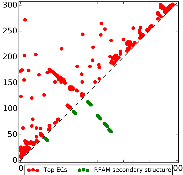
Top L contacts for RF01849 with |i-j| > 4
