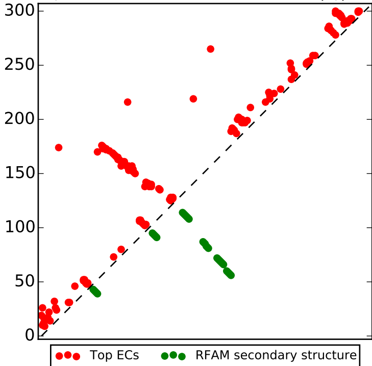
Top L/2 contacts for RF01849 with |i-j| > 4
