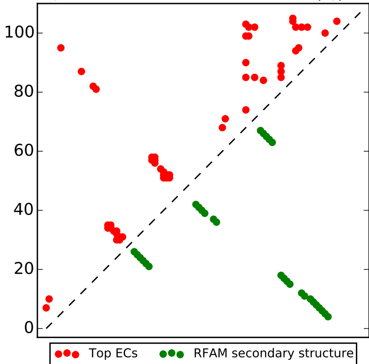
Top L/2 contacts for RF01853 with |i-j| > 4
