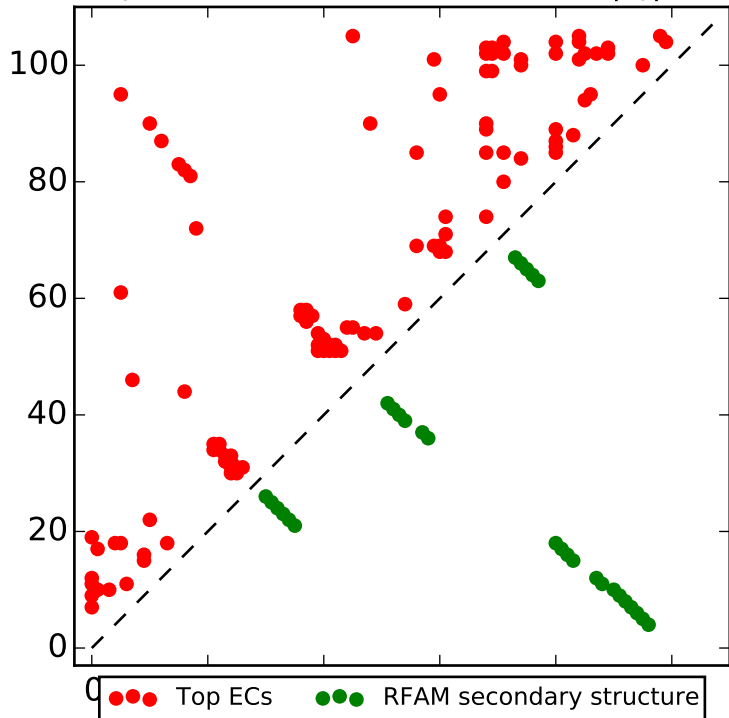
Top L contacts for RF01853 with |i-j| > 4
