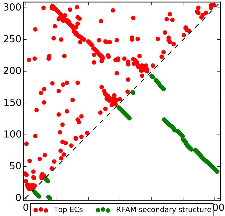
Top L contacts for RF01855 with |i-j| > 4
