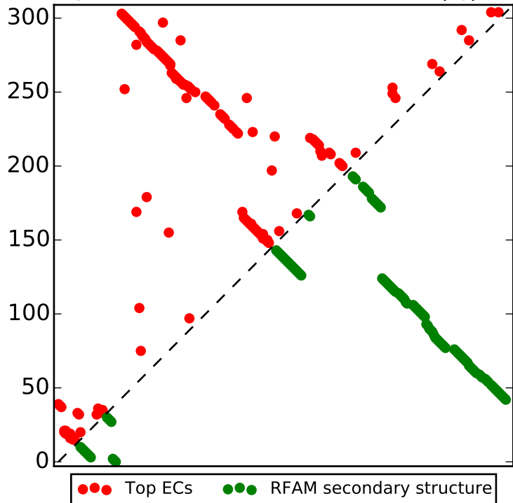
Top L/2 contacts for RF01855 with |i-j| > 4
